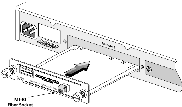
Figure 1 Inserting the Module into the Switch
