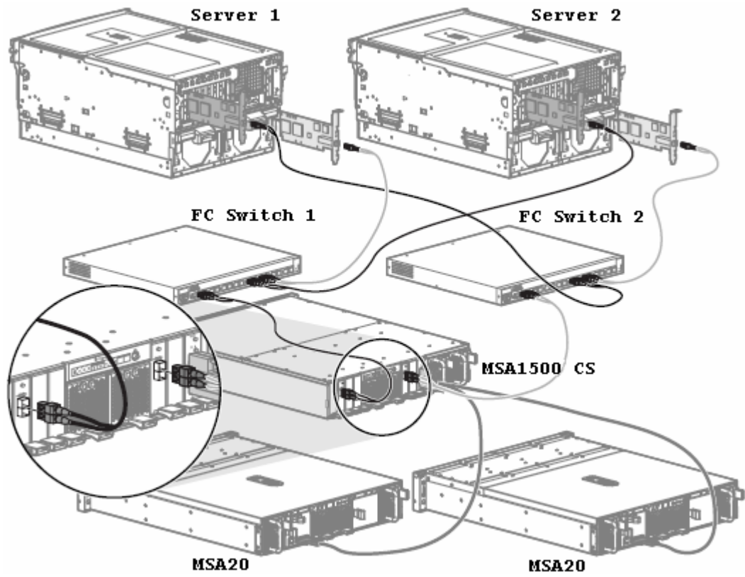
Figure 5. A Typical Multi-Path Configuration
