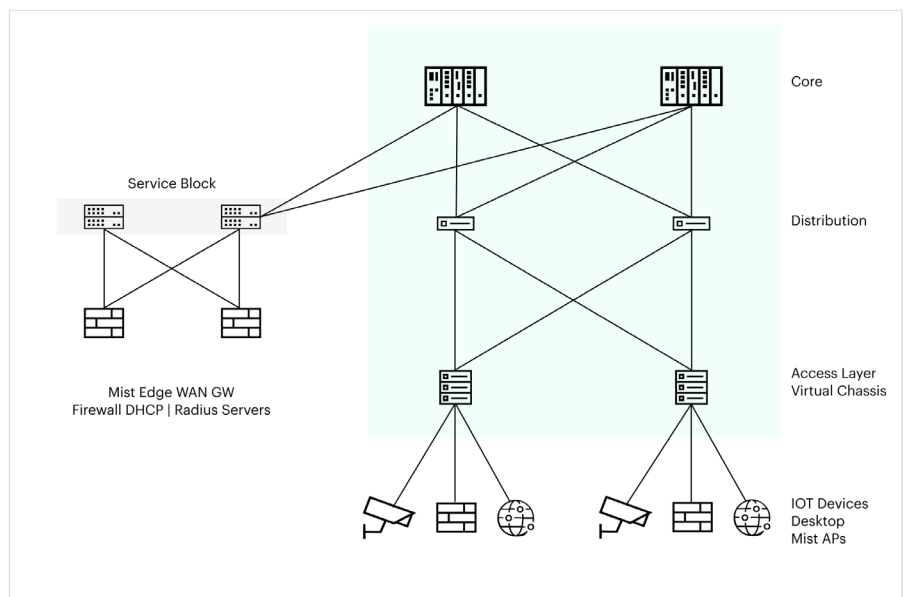
Figure 1. The Campus Fabric IP Clos JVD solution
