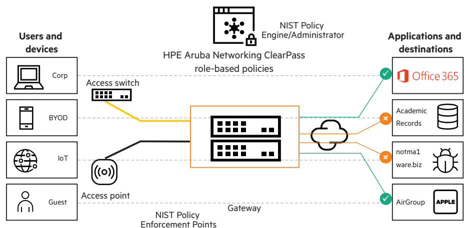
Figure 1. Trust enforced by HPE Aruba Networking dynamic segmentation
