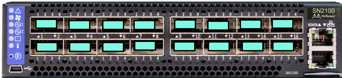
All 16 QSFP28 ports 1-16 support x4 or x2 breakout
