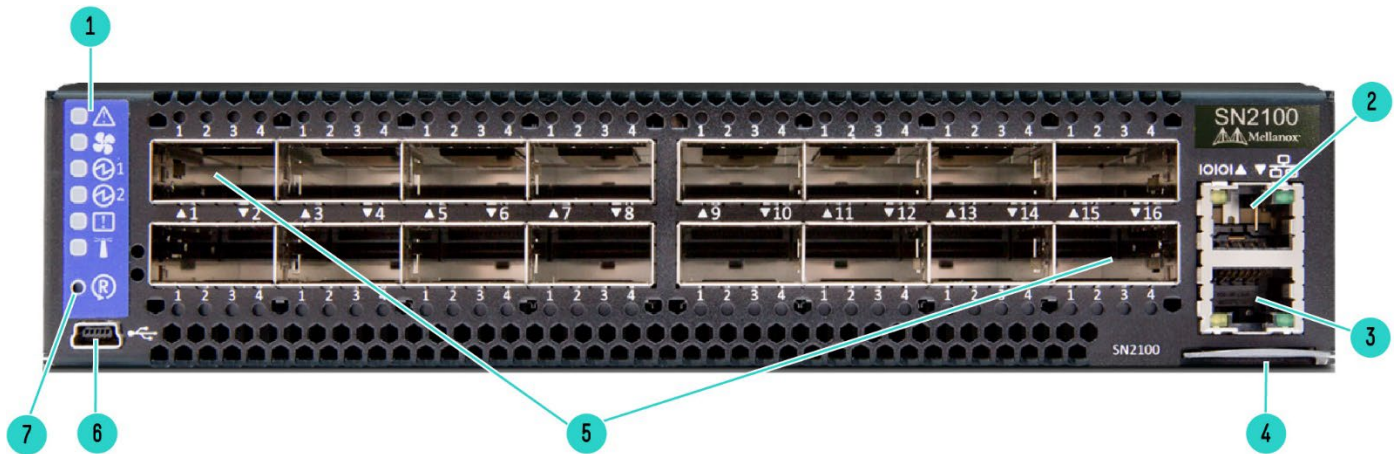
HPE Storage Switch M-series SN2100M Front View
