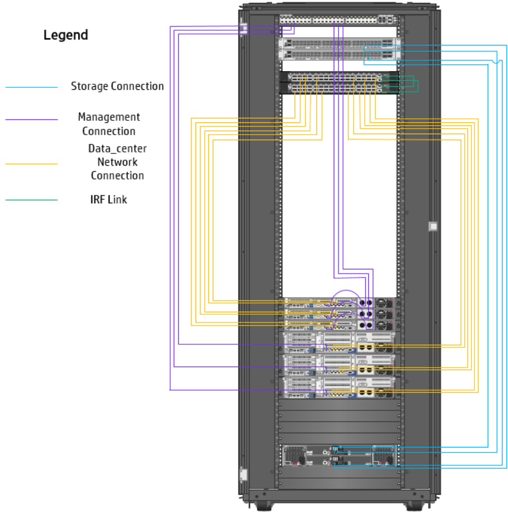
FIGURE 9. Rack Network wiring connections of servers, storage, and network devices
