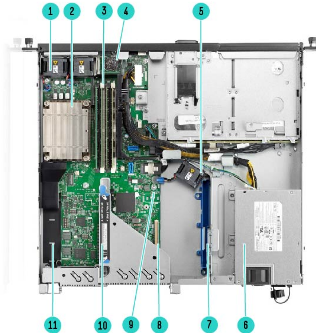
Internal View - Standard for all DL20 Gen10
