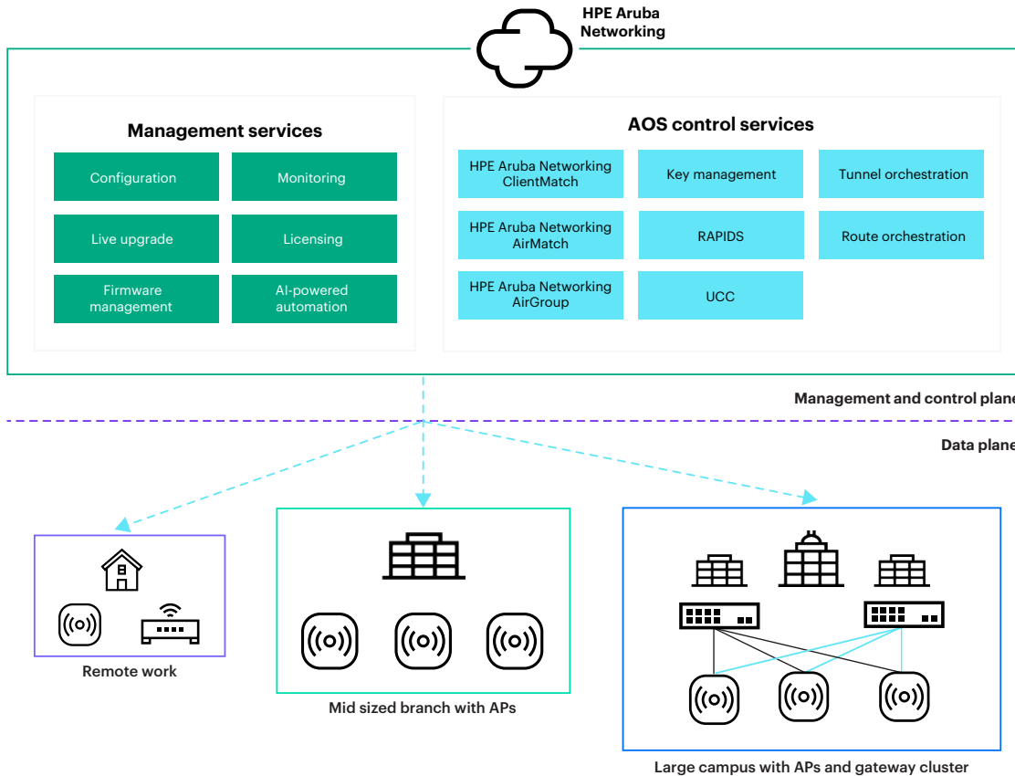
Figure 1. Distributed HPE Aruba Networking Wireless Operating System 10 supports APs and optional gateways
