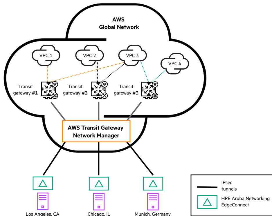
Figure 1. Branch-to-Cloud and Branch-to-Branch Connectivity using AWS TGNM
