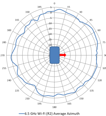
Figure 3. 6.5 GHz Wi-Fi antenna patterns (horizontal)
