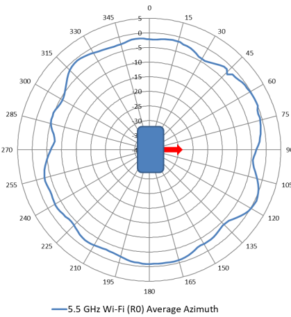
Figure 2. 5.5 GHz Wi-Fi antenna patterns (horizontal)
