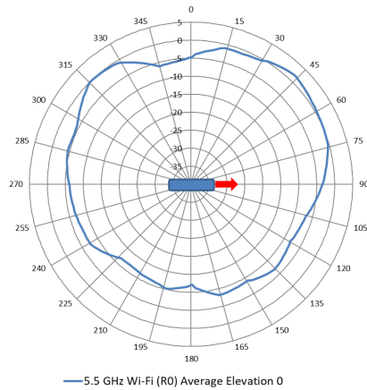
Figure 6. 5.5 GHz Wi-Fi antenna patterns (vertical) with elevation 0
