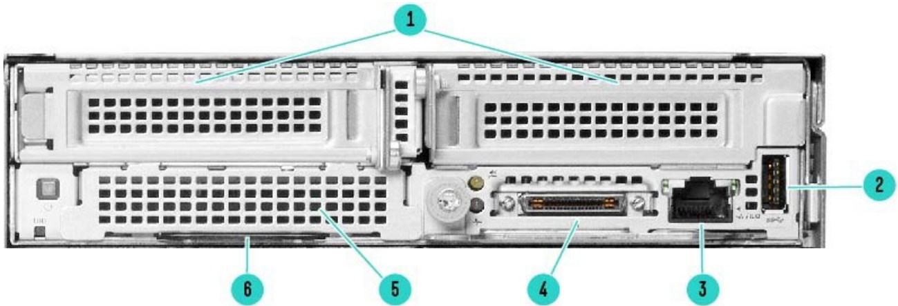
HPE ProLiant XL22Xn Gen10 Plus Server Rear Panel Components
