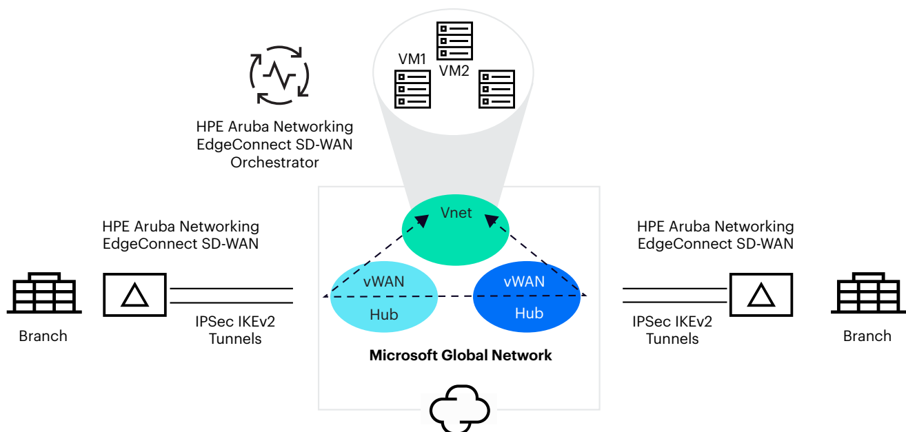
Figure 4. Branch-to-Cloud and Branch-to-Branch connectivity using Azure vWAN
