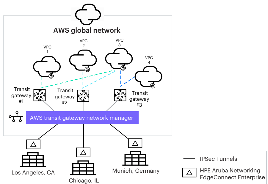
Figure 3. Branch-to-cloud and branch-to-branch connectivity using AWS TGNM
