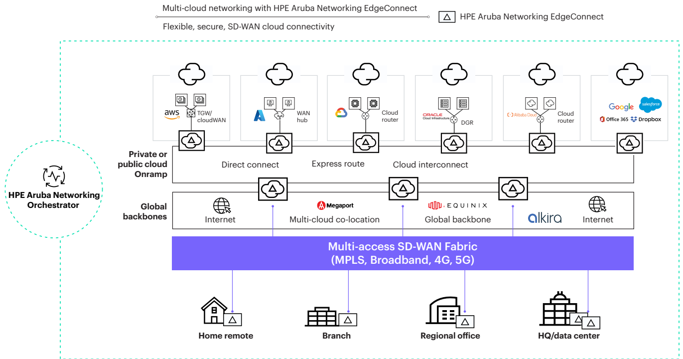
Figure 6. Flexible Multi-Cloud Deployment with EdgeConnect Enterprise SD-WAN
