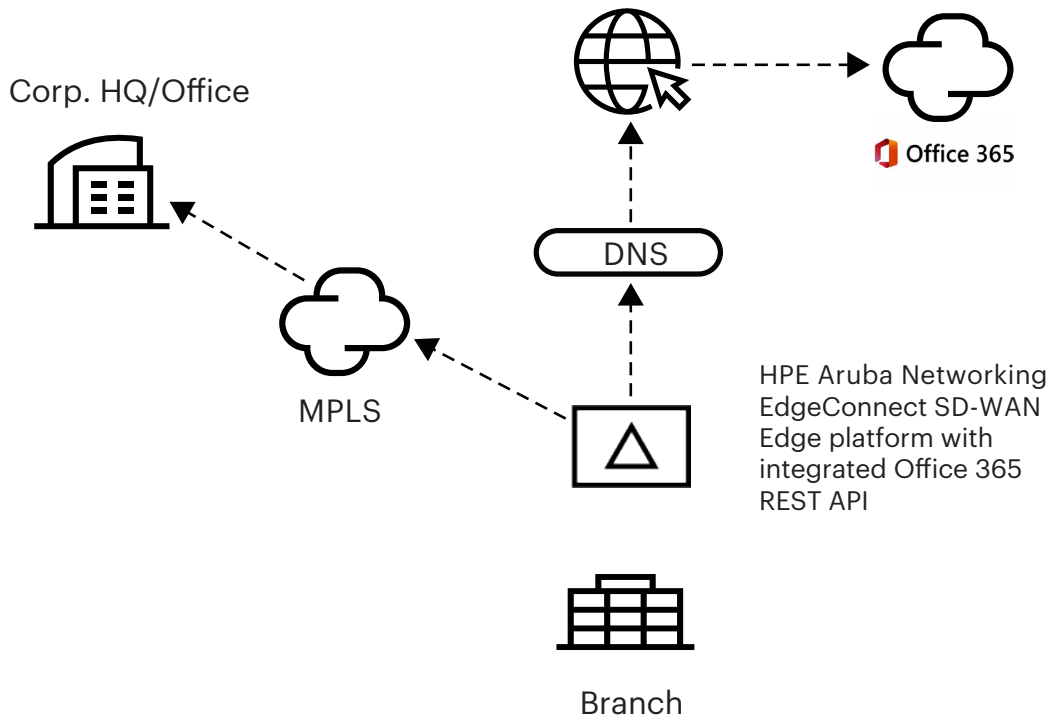
Figure 5. HPE Aruba Networking EdgeConnect SD-WAN enables secure internet breakout directly from the branch office to the closest Office 365 entry point using the latest Office 365 endpoint data
