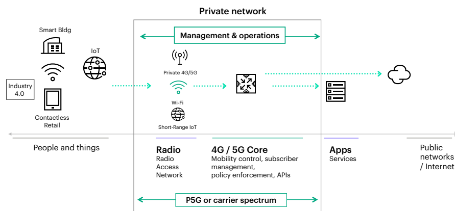
Figure 1. Key components of a private 4G/5G cellular network
