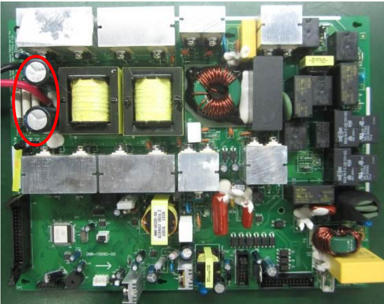
Electrolytic Capacitors >2.5cm dia/height
