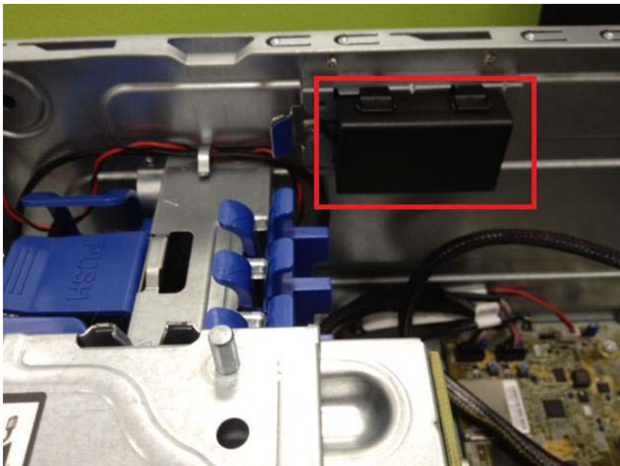
Remove Capacitors
