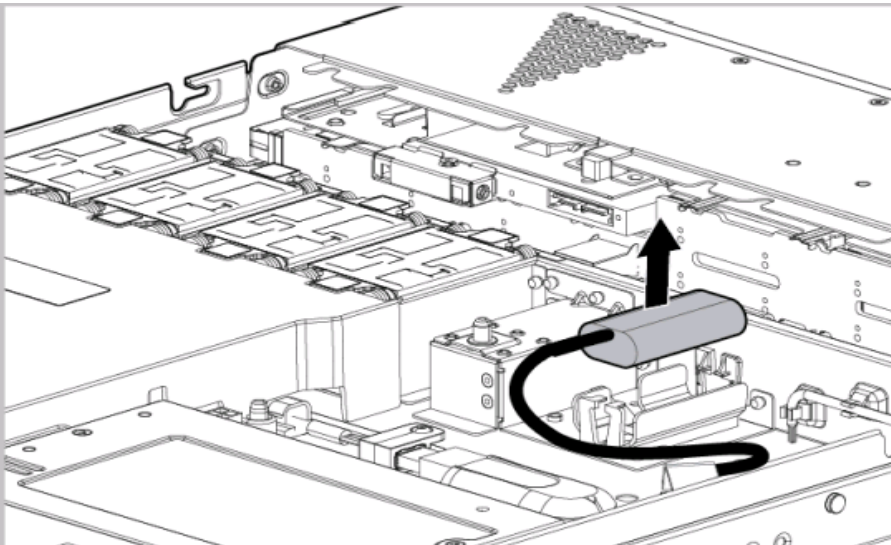
Remove Capacitors
