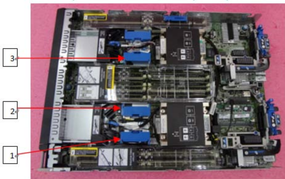
Remove Capicators
