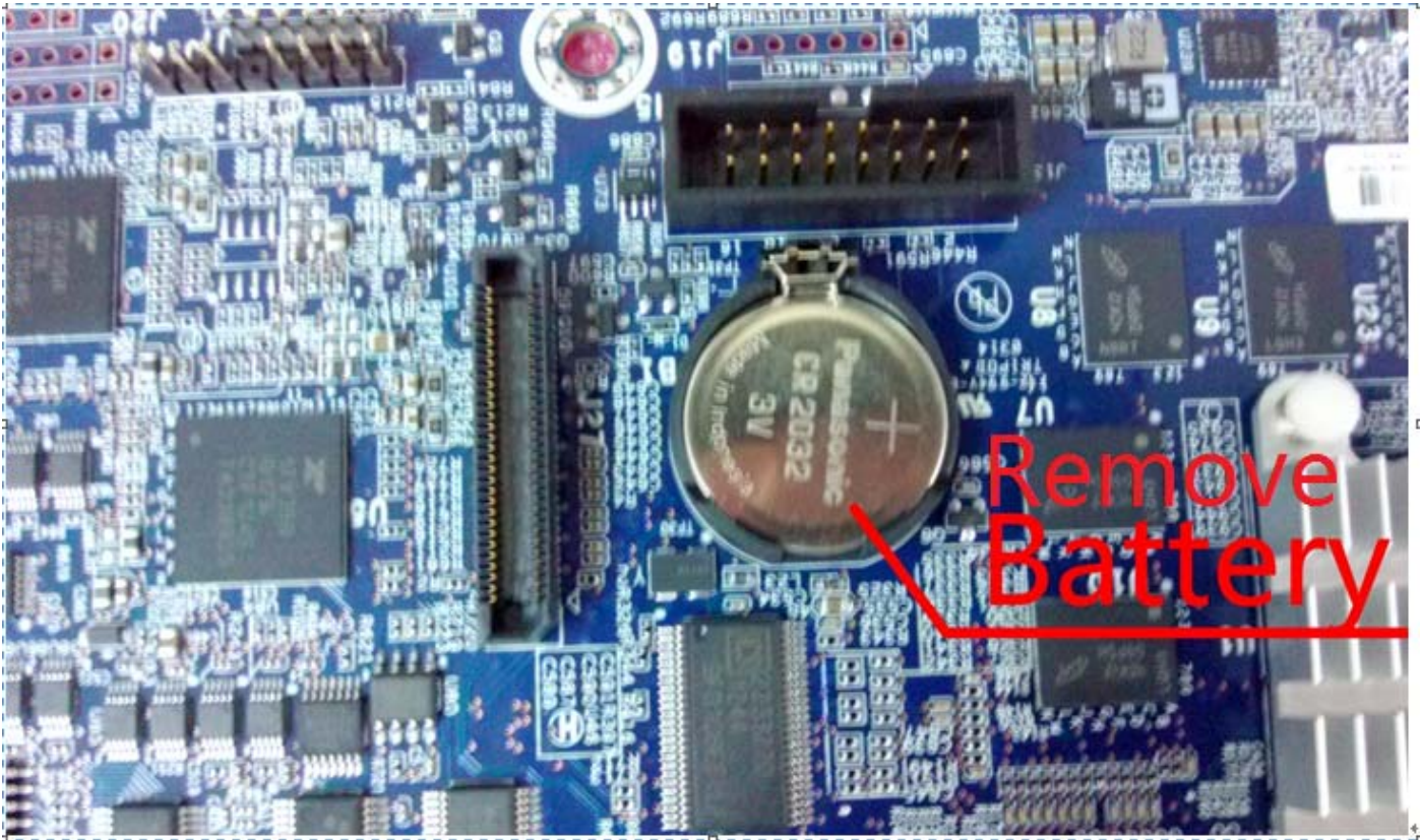
Attachment 3: System Battery Location
