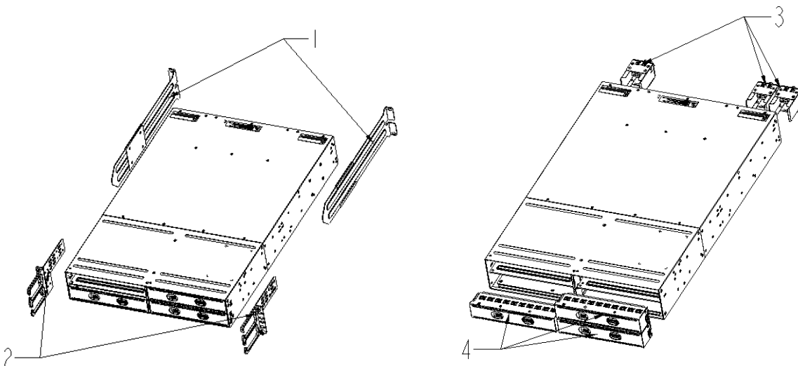
Figure 1 Remove mounting angle Figure 2 Remove blank panel
