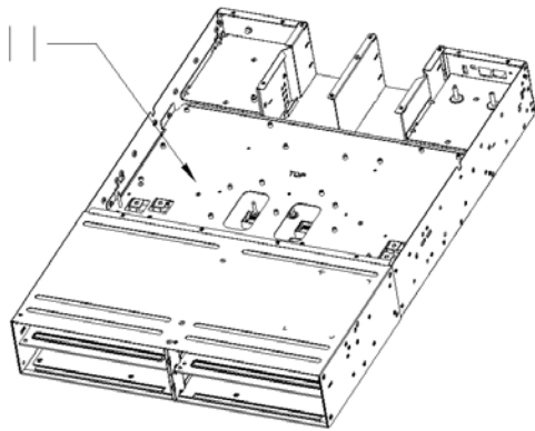
Figure 5 Remove PCB bracket
