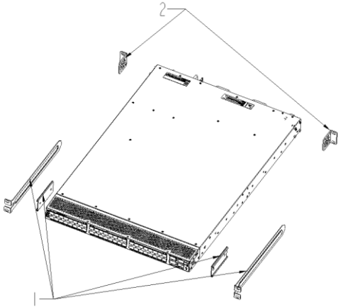
Figure 1 Remove mounting angle
