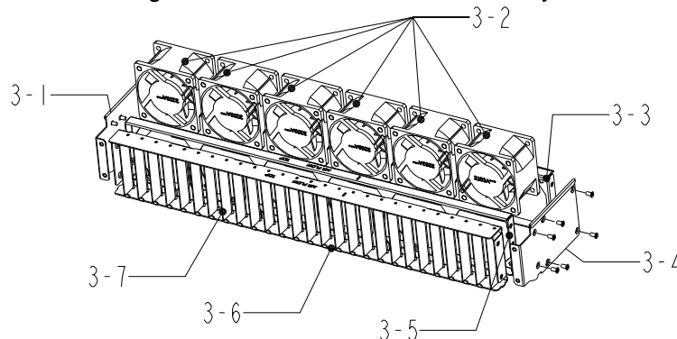
Figure 2 Treatments to assembly 3
