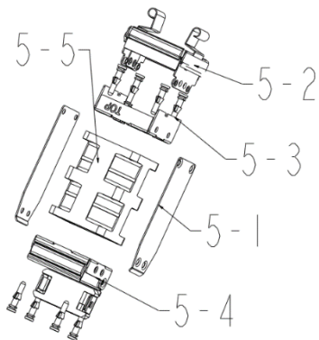
Figure 5 Treatments to fan-assembly
