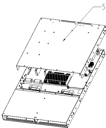
Figure 3 Remove top cover
