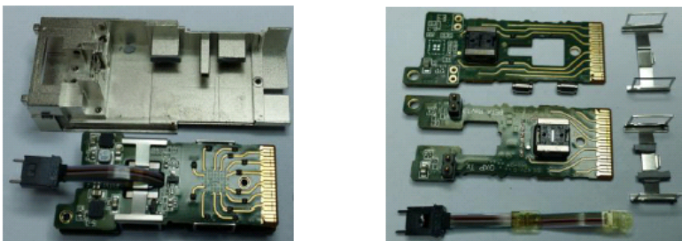
Figure 1 CXP Module Dis-assembly
