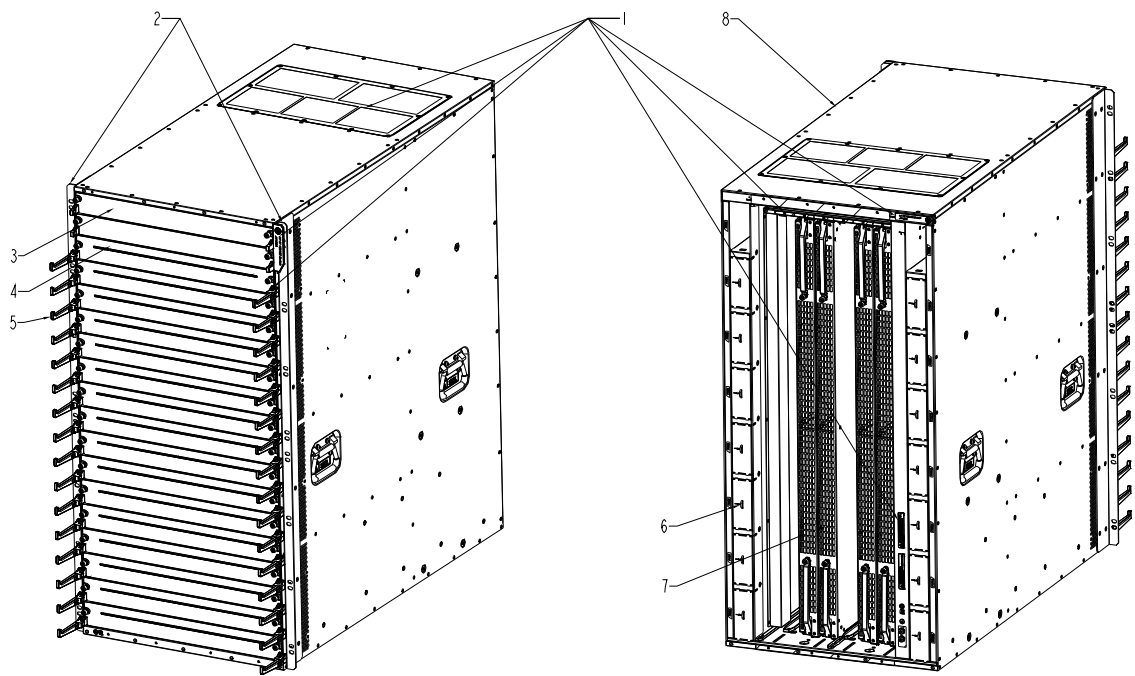
Figure 1Overall view of the product
