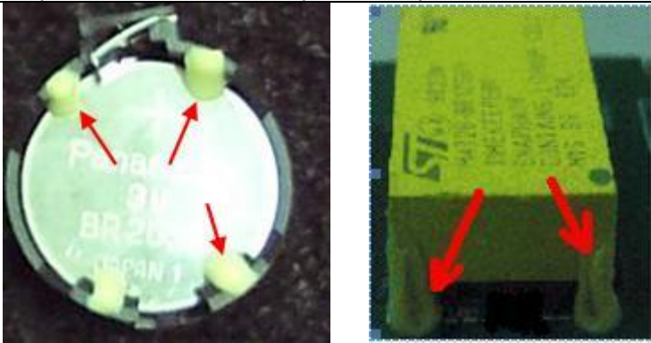
Figure 2 Clear the yellow adhesives by the tweezers.
