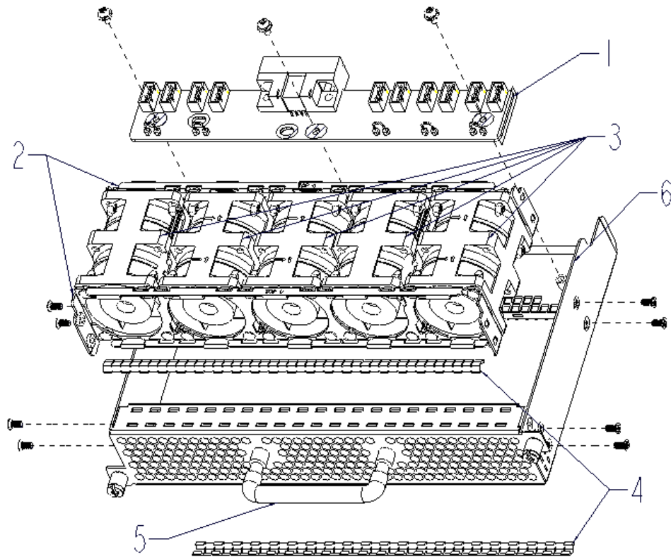
Figure 1 Treatments to fan-assembly
