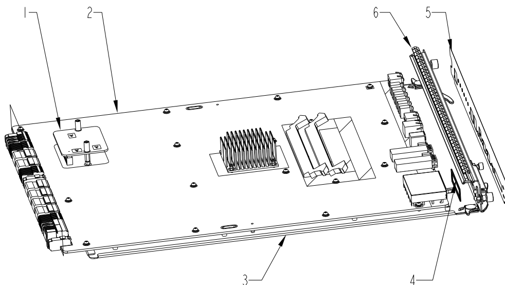
Figure 1 Explode View of the Front Panel
