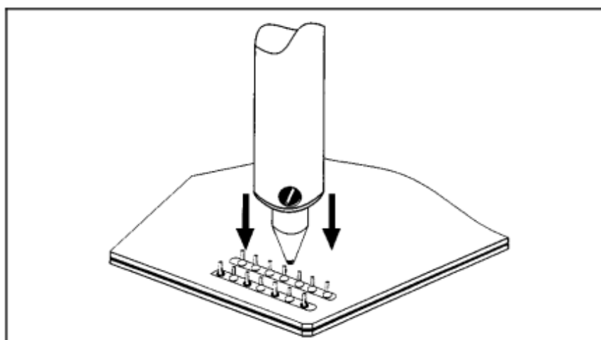
Figure 2 Position Tip
