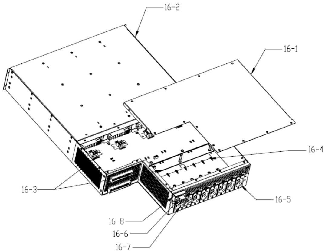
Figure 10 Treatments to power chassis 16
