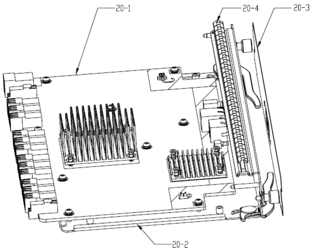
Figure 13 Treatments to panel 20
