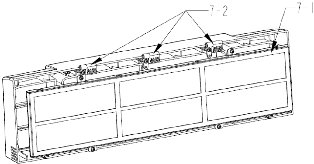
Figure 8 Treatments to plastic panel 7
