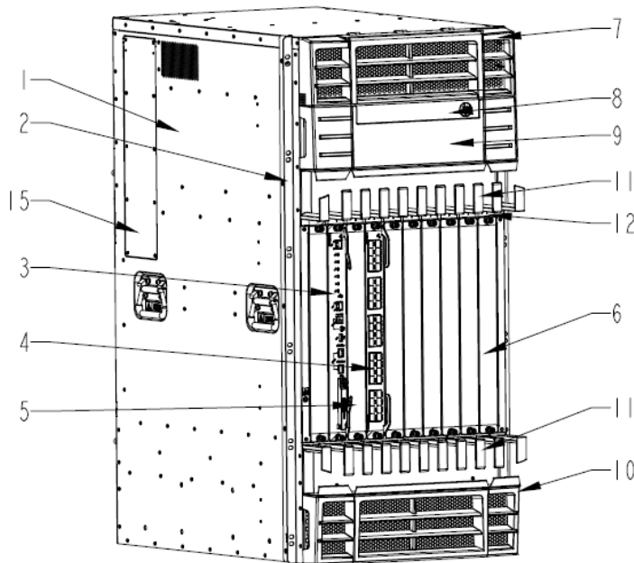
Figure 1 Treatments to the product (front view)
