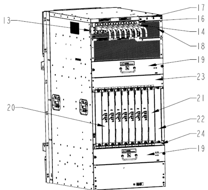
Figure 2 Treatments to the product (rear view)
