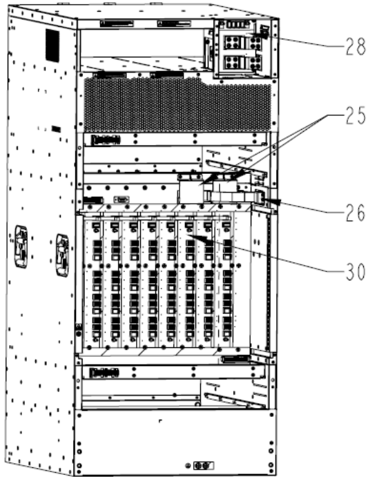
Figure 3 Remove the backboard (rear view)
