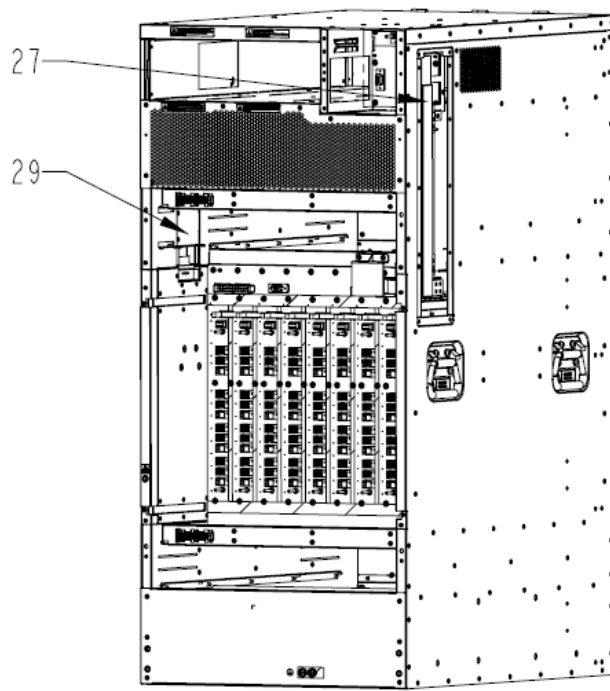
Figure 4 Remove the backboard (rear view)
