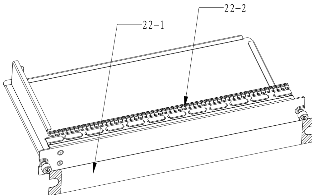
Figure 14 Treatments to panel 22
