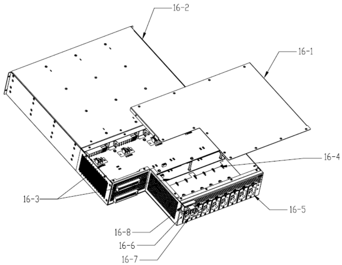
Figure 10 Treatments to power chassis 16
