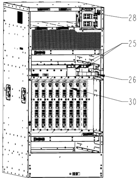
Figure 3 Remove the backboard (rear view)
