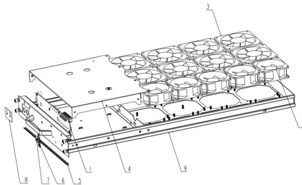
Figure 1 disassembly process
