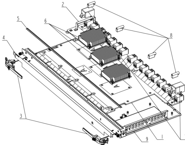
Figure 1 disassembly process
