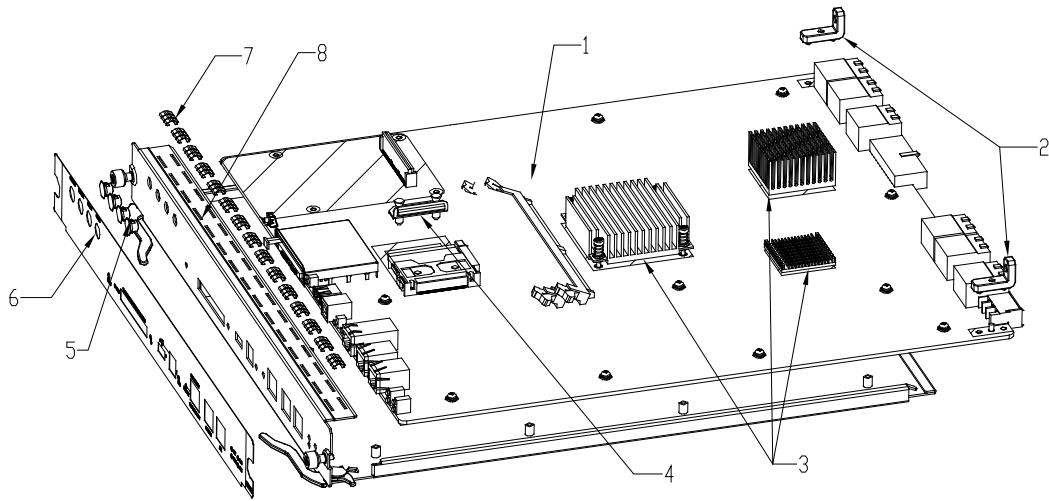
Figure 1 Explode View of the Front Panel
