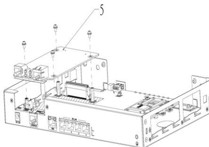
Figure 2 Remove part 2
