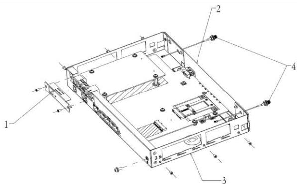
Figure 1 Remove part 1
