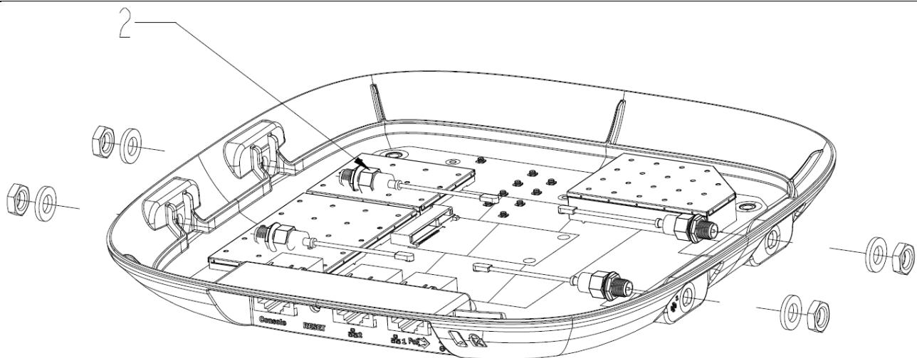
Figure 3 Remove the RF cable
