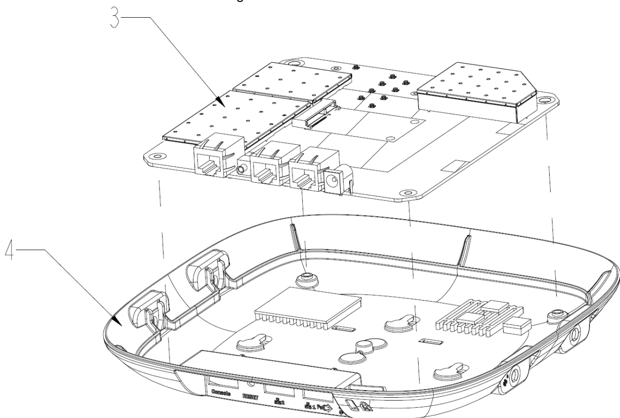
Figure 4 Remove the PCB
