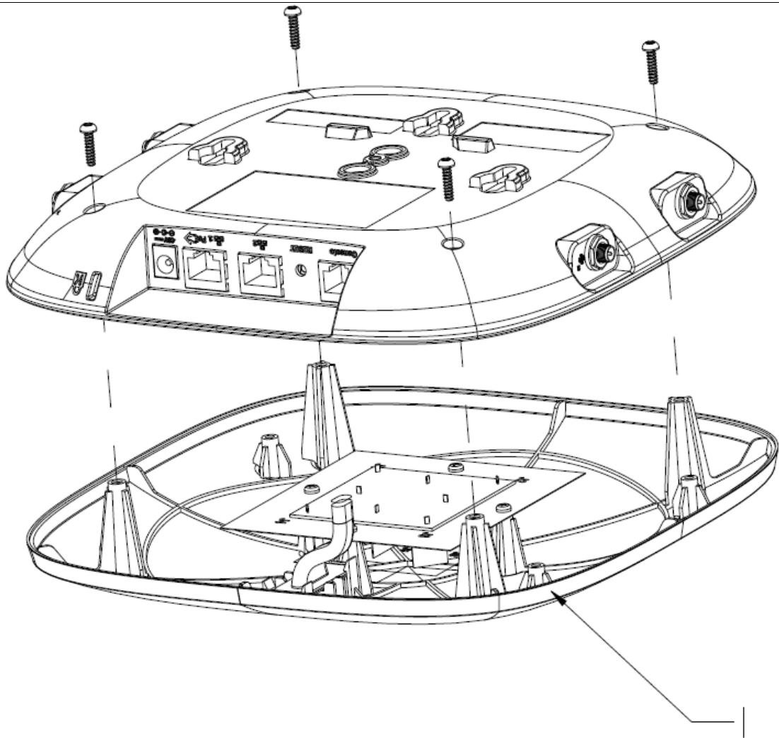
Figure 1 Remove the top cover
