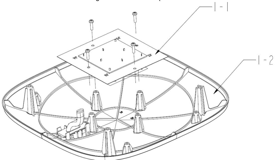
Figure 2 Remove the antenna
