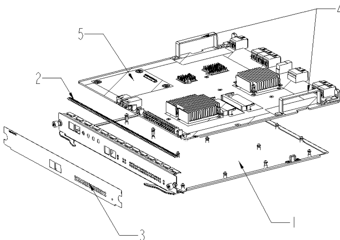
Figure 1 disassembly process
