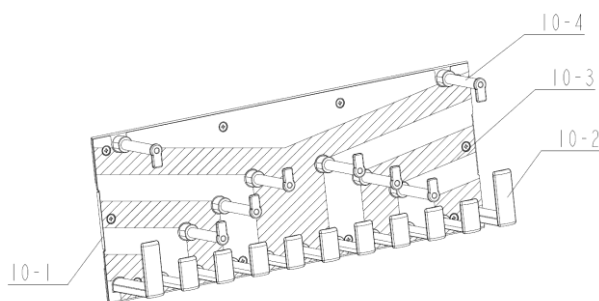
Figure 8 Treatments to upper wire channel sets 10
