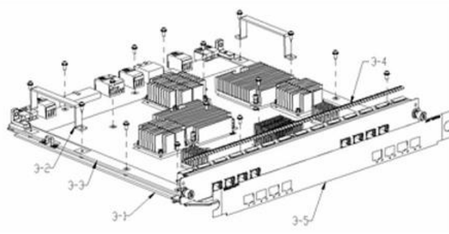
Figure 4 Treatments to front panel 3.
