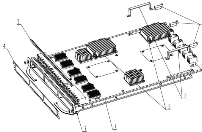
Figure 1 disassembly process
