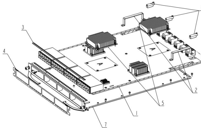
Figure 1 disassembly process
