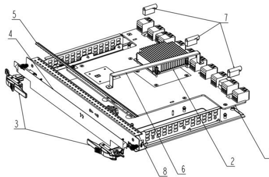
Figure 1 disassembly process
