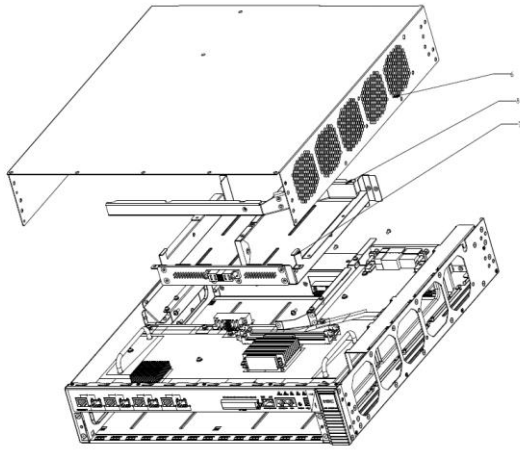
Figure 3 Remove the top cover 6 and power bracket 7
