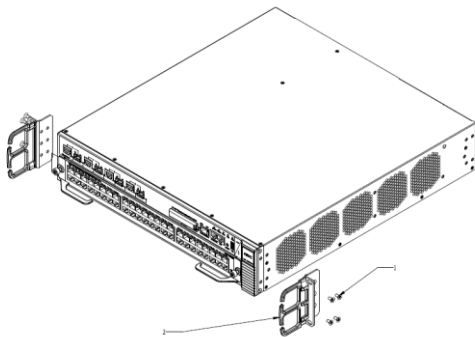
Figure 1 Unscrew screw 1 and the mounting angle 2
