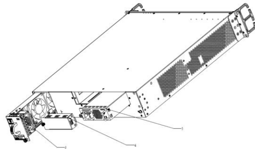
Figure 2 Remove Fan assembly 3 and power 4,5
