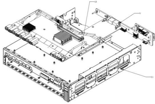
Figure 4 Remove PCB 9 and PCB 10
