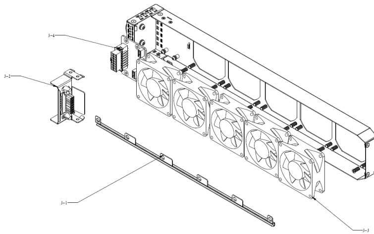
Figure 5 Treatments to Fan assembly 3
