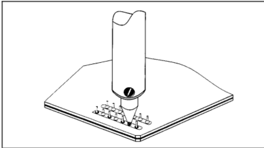
Figure 3 Melt Solder
