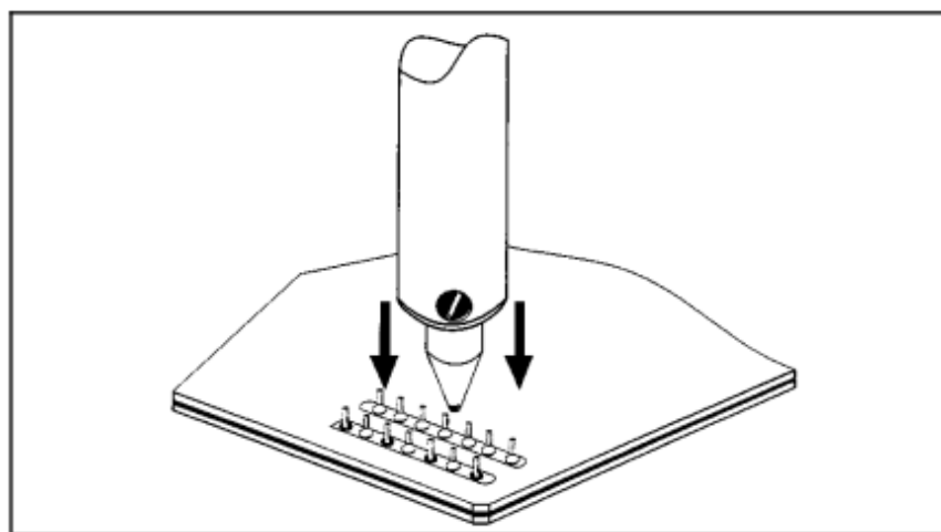
Figure 2 Position Tip
