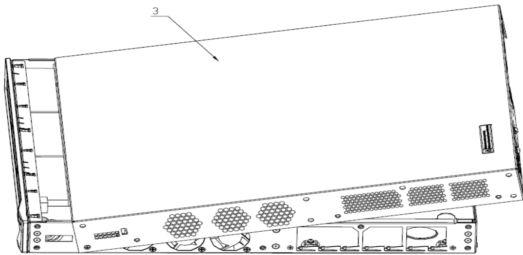
Figure 3 Remove cover
