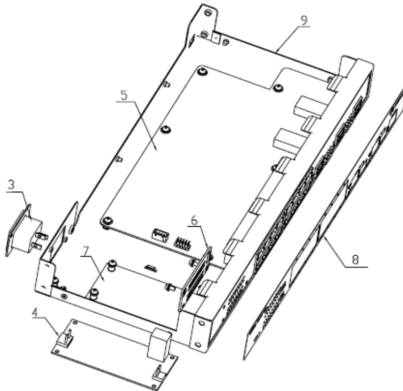
Figure 3 Treatments to the product (remove cover)
