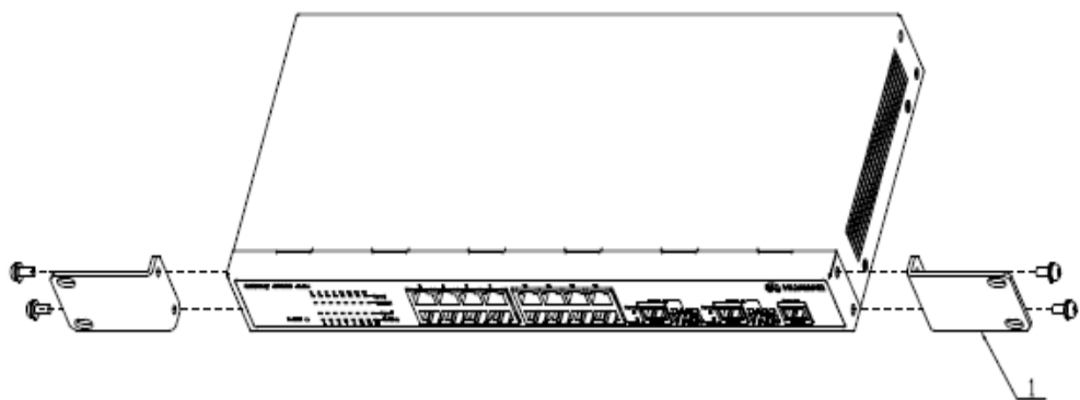
Figure 1 Remove mounting angle
