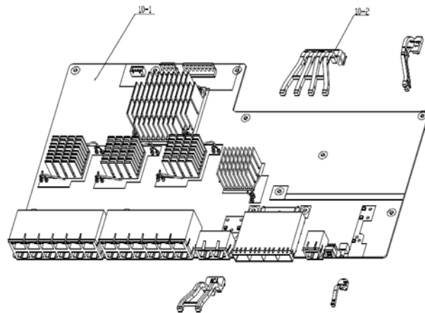
Figure 5 Treatments to PCB 10
