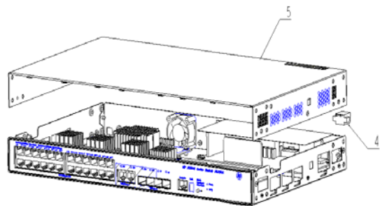
Figure 2 Remove Part 4 and Cover 5
