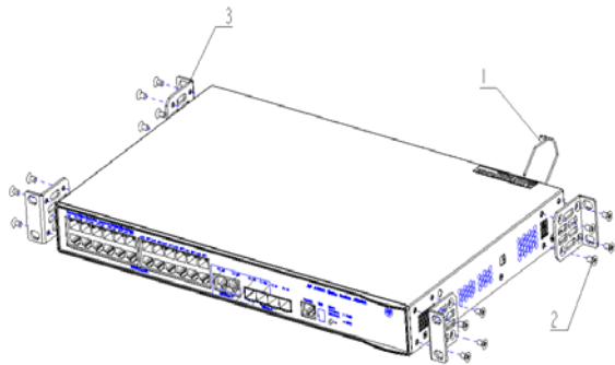
Figure 1 Unscrew the Power Cable Holder 1 and screw 2
