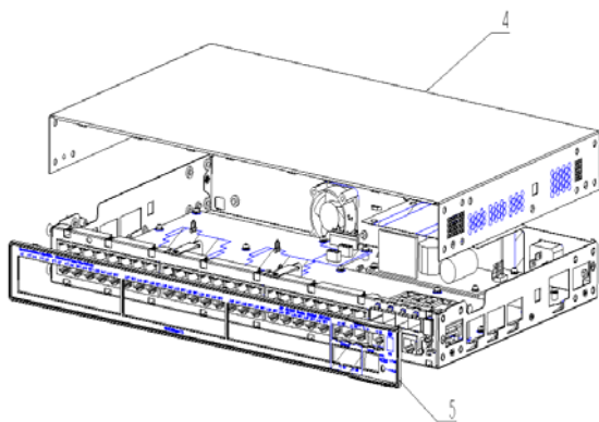
Figure 2 Treatments to the product (rear view)
