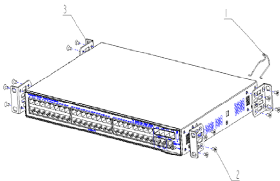
Figure 1 Unscrew the Power Cable Holder 1 and screw 2
