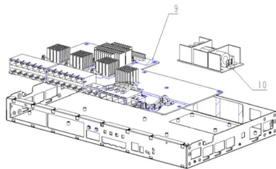
Figure 4 Remove PCB 9 and part 10
