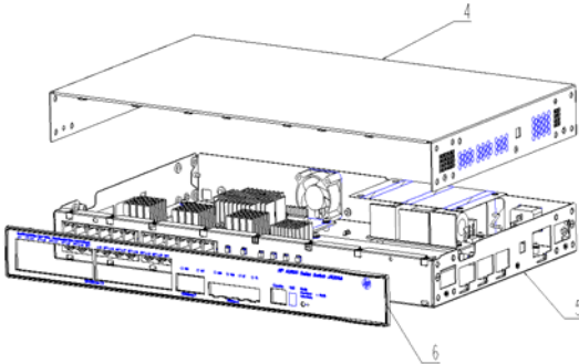
Figure 2 Remove cover 4 and plastic panel 6
