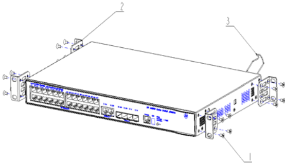
Figure 1 Unscrew screw 1 and the Power Cable Holder 3
