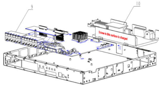
Figure 4 Remove the PCB and Power Module
