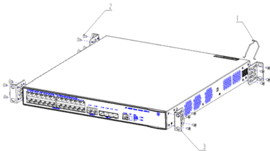
Figure 1 Unscrew the Power Cable Holder 1 and screw 2
