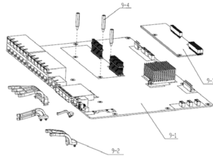
Figure 6 Treatments to PCB 9
