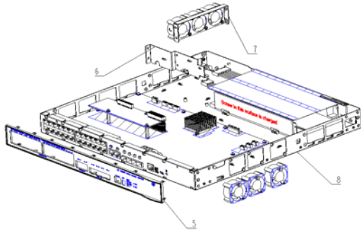
Figure 3 Remove the fan rack, plastic panel 5 and part 6
