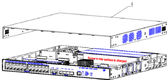
Figure 2 Remove Cover 4
