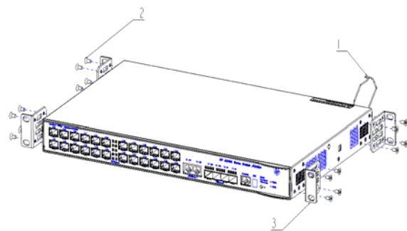
Figure 1 Unscrew the Power Cable Holder 1 and screw 2
