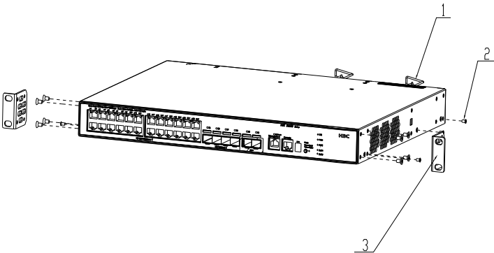
Figure 1 Unscrew the Power Cable Holder 1 and screw 2
