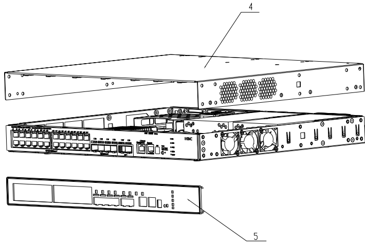
Figure 2 Remove Part 4 and Cover 5
