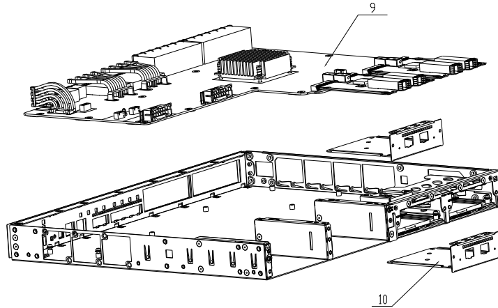
Figure 4 Treatments to the product(II)
