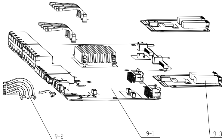
Figure 5 Treatments to PCB 9
